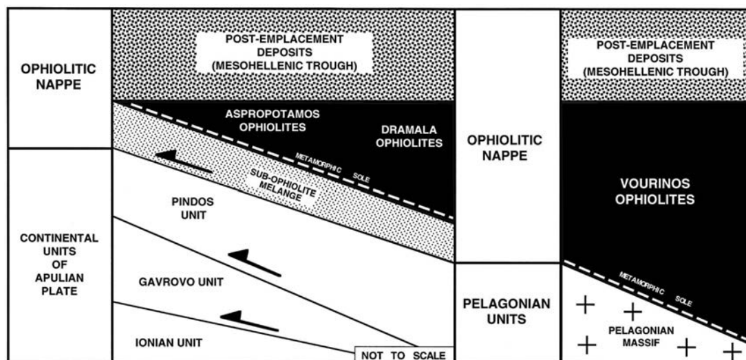
Fig. 5 - Sketch of the tectonic setting of Pindos and Vourinos areas (Greece).
