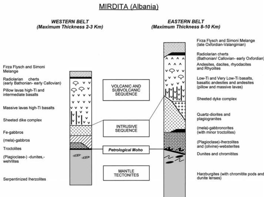
Fig. 4 - Generalised stratigraphy of the ophiolite sequences for the Western and Eastern belt (Modified after Bortolotti et al., 1996).
