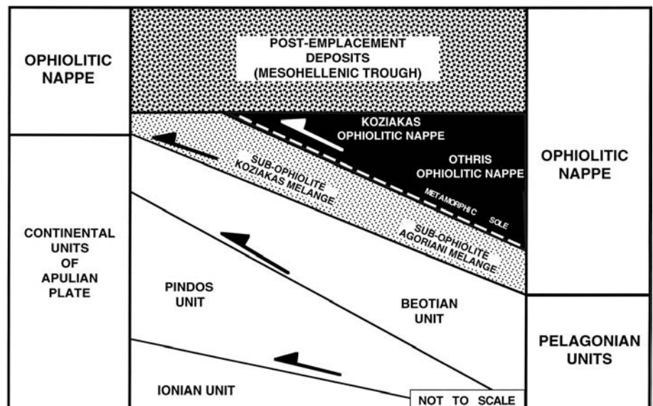
Fig. 8 - Sketch of the tectonic setting of Koziakas and Othris areas (Greece).
