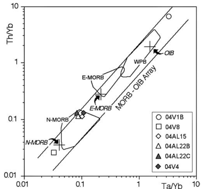
Fig. 8 - Th/Yb vs. Ta/Yb diagram Th/Yb vs. Ta/Yb diagram for volcanic rocks from the Rubik Complex and Porava Unit from southern Albania. Modified after Pearce (1983). Compositions (crosses) of Modern normal mid-ocean ridge basalt (N-MORB), enriched mid-ocean ridge basalt (E-MORB) and within-plate ocean island basalt (OIB) are from Sun and McDonough (1989). Compositional fields of Triassic E-MORBs and within-plate basalts (WPB), as well as Triassic and Jurassic N-MORBs from various sub-ophiolitic mélangé units from the Albanide-Hellenide belt (Saccani and Photiades, 2005) are reported for comparison.
