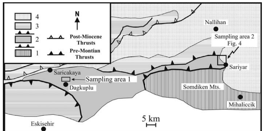
Fig. 2 - Simplified map of the main structural units in the Central Sakarya area (after Göncüoğlu et al., 2000). Explanations: 1- Somdiken Metamorphics (Tauride-Anatolide Platform); 2- Central Sakarya Ophiolitic Complex, 3- Sakarya Composite Terrane; 4- Tertiary Cover.
