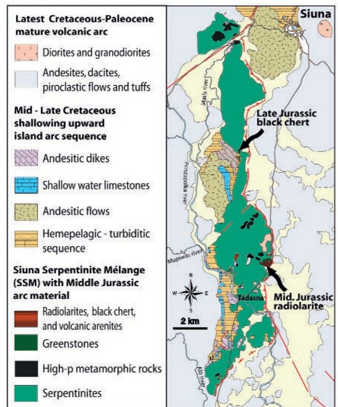
Fig. 2 - Geologic map of the Siuna area, showing the Siuna Serpentine Mélange and its tectono-stratigraphic context. The two radiolarian sample localities are indicated. Geology partially after Venable (1994).
