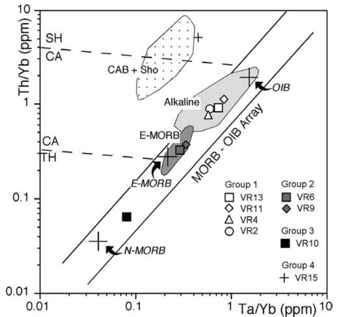
Fig. 5 - Th/Yb vs. Ta/Yb diagram for volcanic rocks from the mélange. Large crosses indicate the compositions of Modern ocean-island basalt (OIB), enriched-type mid-ocean ridge basalt (E-MORB), and normal-type mid-ocean ridge basalt (N-MORB), according to Sun and McDonough (1989). Variations of elemental ratios of Triassic calc-alkaline basalts (dotted field), Triassic alkaline basalts (light gray field), and E-MORBs (dark gray field) from various localities of the Hellenides are reported for comparison (data from Pe-Piper and Piper, 2002; Saccani and Photiadis, 2005, and references therein).
