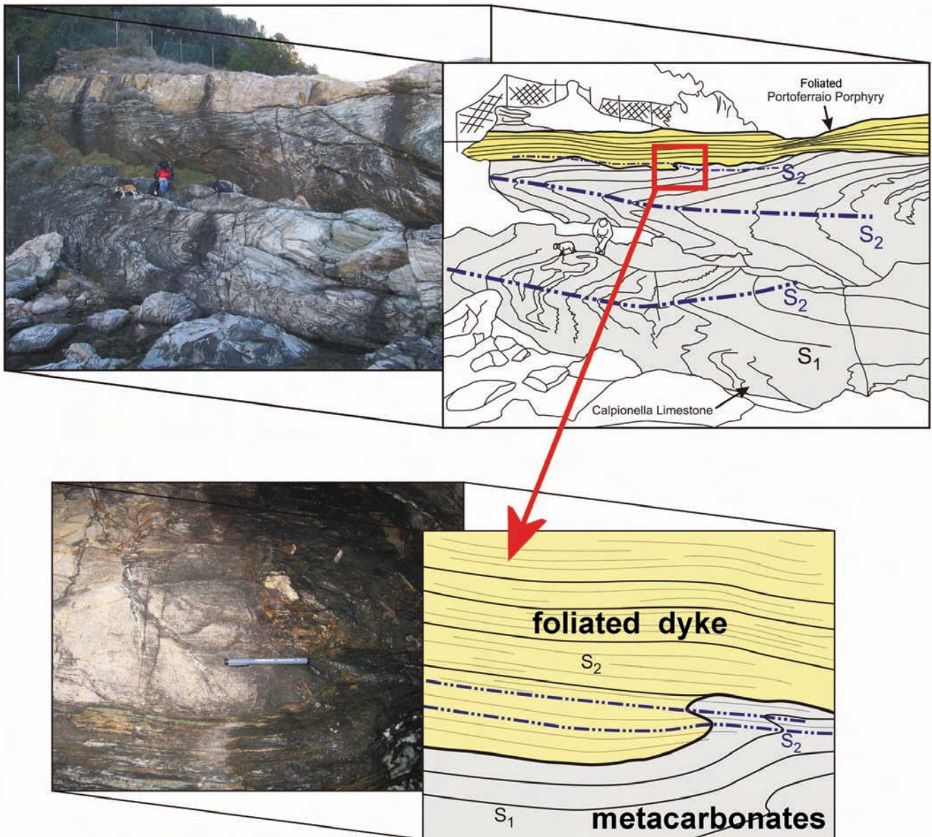
Fig. 6 - Structural features of the Spartaia shear zone. Folded metalimestone including a foliated Portoferraio-type metaporphyritic body (modified from Pandeli et al., 2013).
