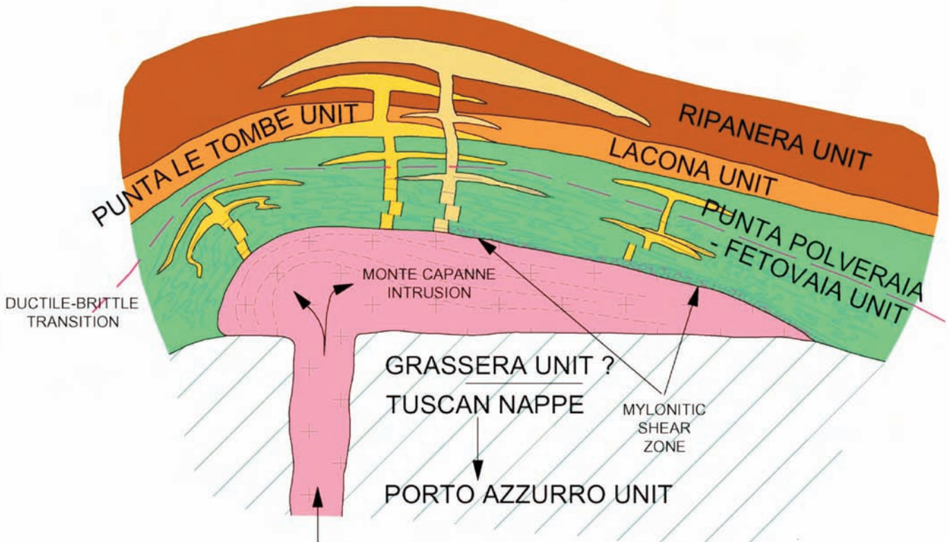
Fig. 13 - Sketch of the forced intrusion of the Mt. Capanne pluton and ductile deformations and shearing in the surrounding PFU successions (modified from Daniel and Jolivet, 1995).
