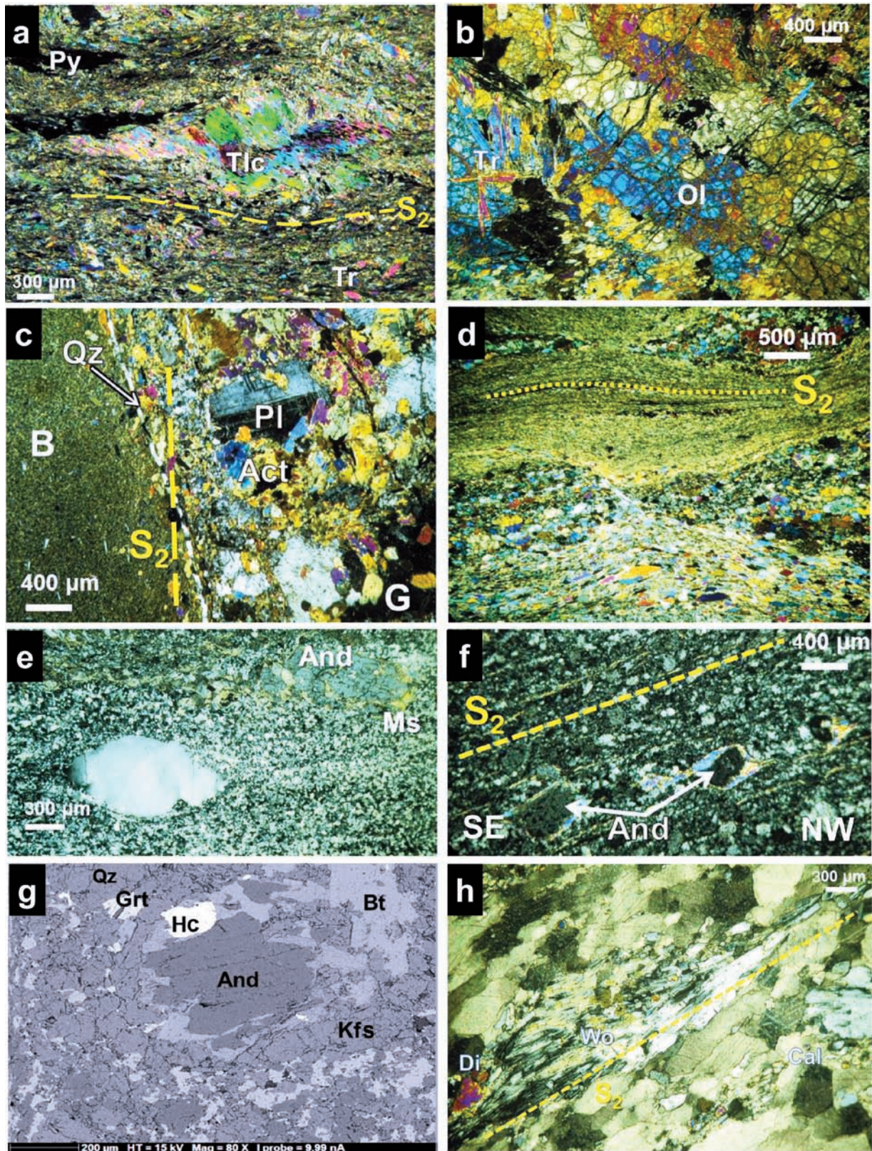
Plate 2 - Photomicrographs of the contact mineralogic assemblages and structures in the rocks of PFU: a) Rotate syn-tectonic Tlc porphyroclast within the main Amp foliation in the serpentinites at Colle Palombaia; b) Neoblastic Ol after cellular Srp in the serpentinites at Punta Nera; c) Foliated contact between metagabbros (G) and metabasalts (B) at Colle Palombaia with a Qz vein; d) Foliated metabasalts at Colle Palombaia; e) Metacherts with And porphyroblasts at Colle Palombaia; f) Mantled And porphyroclasts in the metacherts at Colle Palombaia; g) SEM image of Hc-bearing metacherts at Colle Palombaia; h) Wo and Di lying along the main foliation in the metalimestones at Cavoli-Colle Palombaia; i) Deformed Wo- and Ves-bearing main foliation in the metalimestones at Cavoli-Colle Palombaia; j) Mantled Di porphyroclasts within the main foliation in the exoskarn levels of the metashales and metalimestones at Punta della Fornace (NW of Colle d'Orano); k) Static Wo radiating sphaerule with Di core in the metalimestones at Semaforo locality; l) Wo+Ves in a decarbonated exoskarn of the metalimestones at Cavoli-Colle Palombaia; m) Tur-rich, foliated Portoferraio-type metaporphry at Punta del Timone (North of Chiessi); n) Foliated and sericitized, S.Martino-type metaporphry composite rounded Qz porphyroclasts at Punta del Timone (North of Chiessi).
