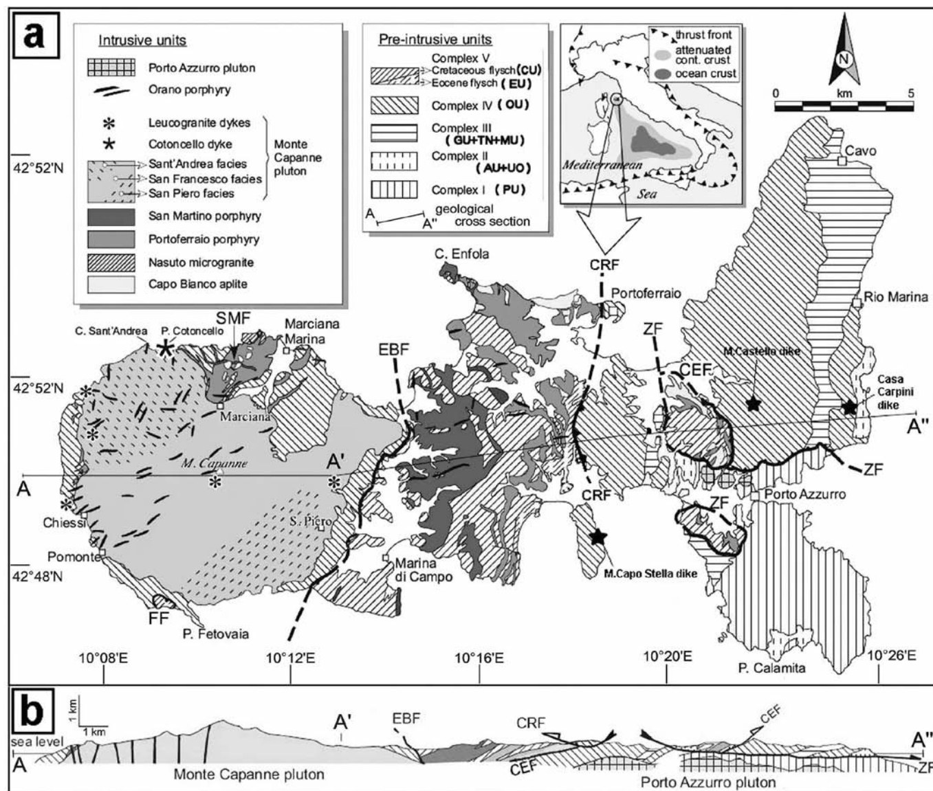
Fig. 1 - Geological map (a) and section (b) of the Elba Island, including the different magmatic bodies (modified from Westerman et al., 2003). EBF- Eastern Border Fault (Colle Palombaia-Procchio Fault in this paper), CEF- Central Elba Fault, ZF- Zuccale Fault, CRF- Colle Reciso Fault, FF- Fetovaia Fault. The correspondence of the five Trevisan's (1950) Complexes with Bortolotti's et al. (2001a) Units is reported in the legend of the pre-intrusive Units: PU- Porto Azzurro Unit; UO- Ortano Unit; AU- Acquadolce Unit; MU- Monticiano-Roccastrada Unit; TN- Tuscan Nappe; GU- Gràssera Unit; OU- Monte Strega Unit; EU- Lacona Unit; CU- Ripanera Unit.
