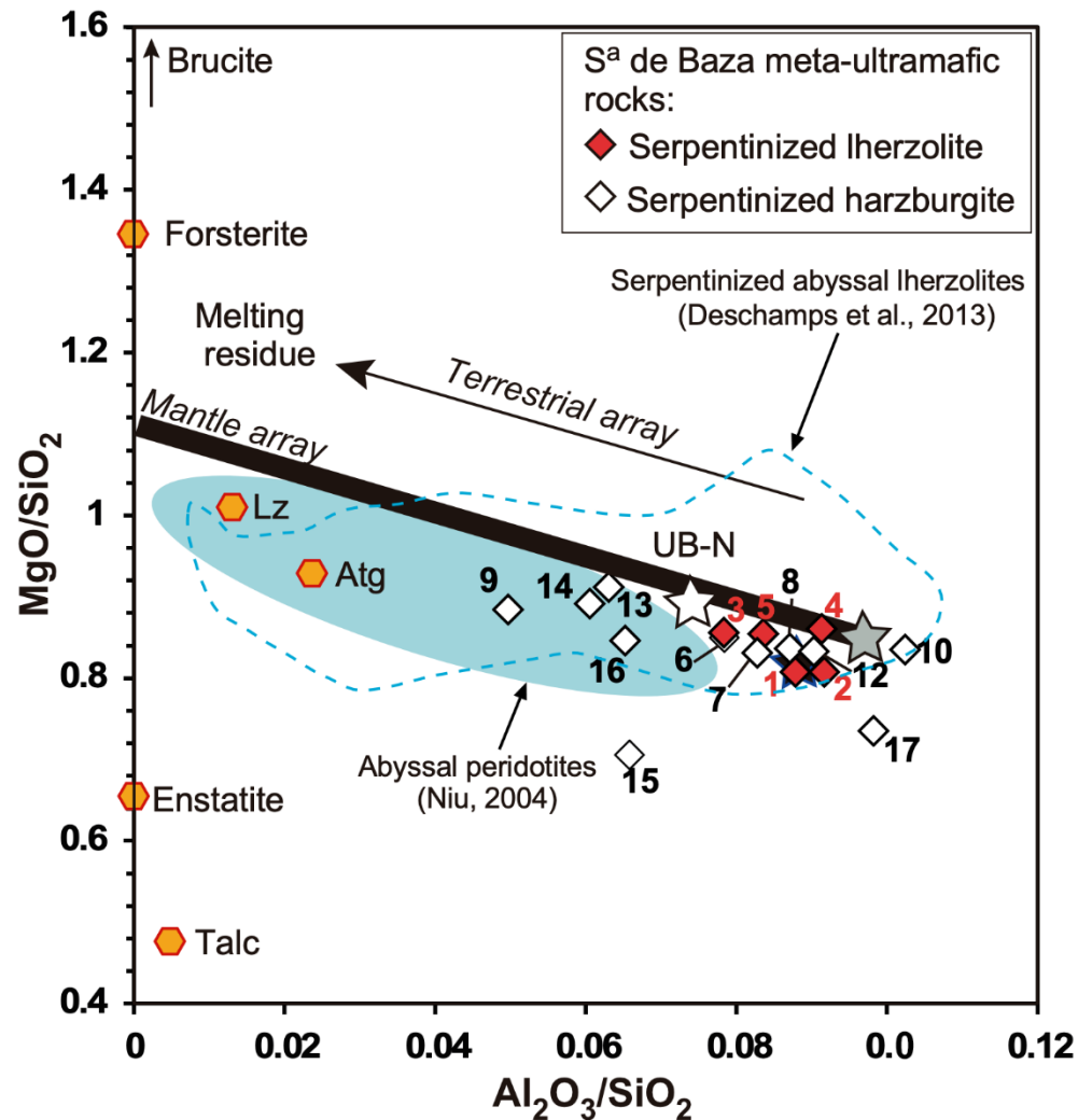
Fig. 3S - \text{Al}_2\text{O}_3/\text{SiO}_2 vs \text{MgO}/\text{SiO}_2 binary diagram for the serpentinites of Sierra de Baza. Estimated composition of the depleted mantle from Salters and Stracke (2004) and primitive mantle from McDonough and Sun (1995). The thick black line represents the massive evolution of silicates on Earth (terrestrial array) from Jagoutz et al. (1979) and Hart and Zindler (1986).
