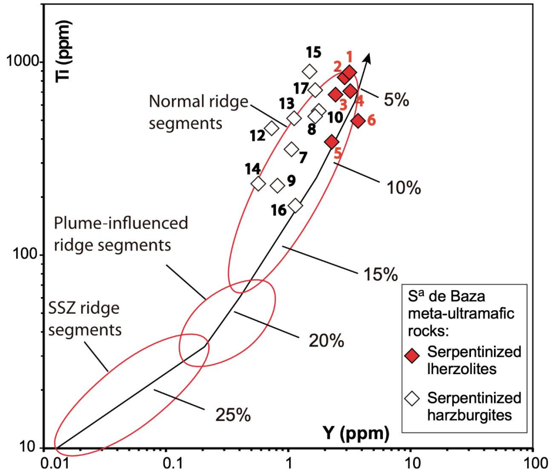
Fig. 4S - Y vs Ti of the Sierra de Baza meta-ultramafic rocks in the discriminant diagram of Pearce and Peate (1995) for peridotites of different tectonic environments. Black line indicates the evolution of mantle composition at various melting degrees.
