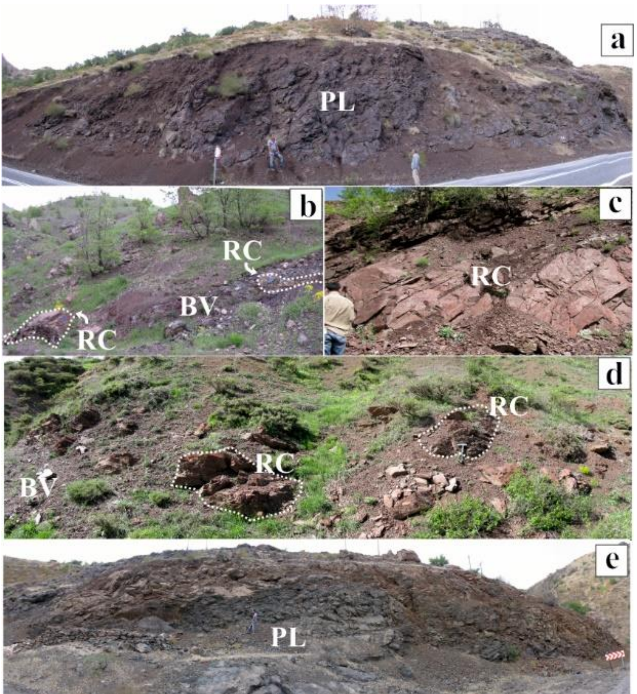
Fig. S1 - Close view of basaltic rocks of Yüksekova Complex, located in the vicinity of the Maden town (SE Elazığ, Turkey), a) Pillowed basaltic volcanics (PL) along the Maden-Diyarbakır main road; Sample MD-10 (x: 555907, y: 425613), b) Radiolarian chert (RC) interlayered with basaltic volcanics (BV) in the Kayalar area, Sample MDN-11 (x: 555507, y: 4256319), c) 2-3 meters thick, reddish radiolarian pelagic cherts (RC); Sample MDN-22 (x: 554392, 4252132), d) Basaltic volcanics intercalated with lenses of radiolarian cherts (RC), Maden-Hazar road; Sample MDN-23 (x: 554392, 4252132), e) basaltic pillow lavas (PL), Zahuran-Maden road, Sample MD-9 (x: 55300, y: 4257530).
