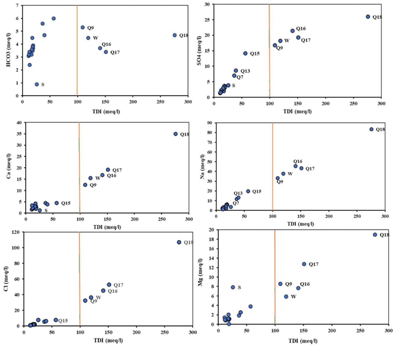
Figure 1S. Bivariate diagrams of distribution of main ions compared to TDI in Naeen aquifer.
