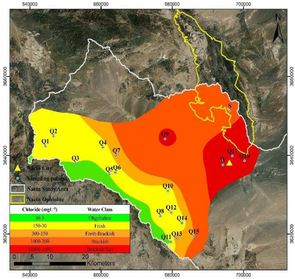
Figure 3S. Changes of Cl - ion concentration in Naeen aquifer
