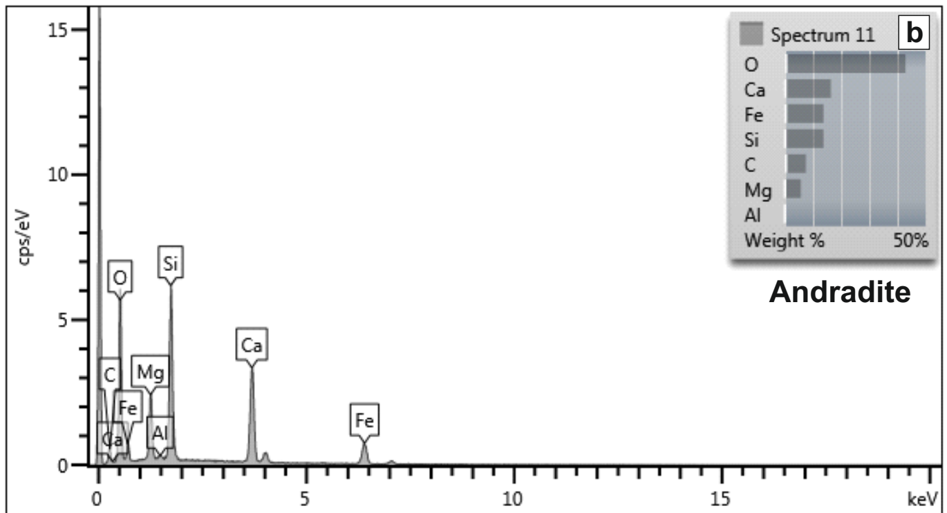
Fig. 1S: (a) Laser-Raman spectrum of the andradite. Red spectrum and the code above show andradite data from RRUFF Raman spectral library used for comparison. (b) Electron dispersive spectrometry (EDS) data from andradite grains.
