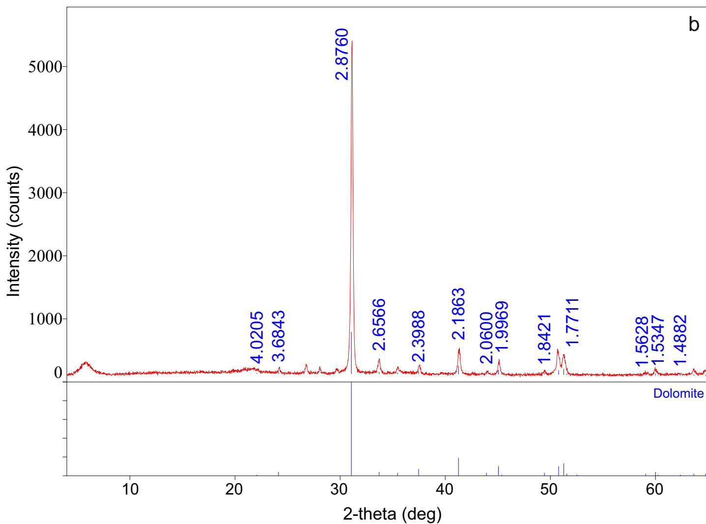
Fig 4S. Whole-rock X-Ray diffraction (XRD) patterns obtained from the lower (a) and upper (b) parts of the iron-oxide stained silica-carbonate alteration crust (Fsc).
